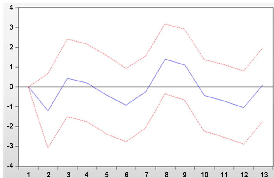
Figure 6. IRF—Exchange rate on copper price.
