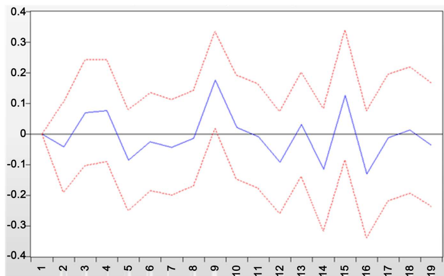
Figure 1. IRF—Copper price on copper production.
