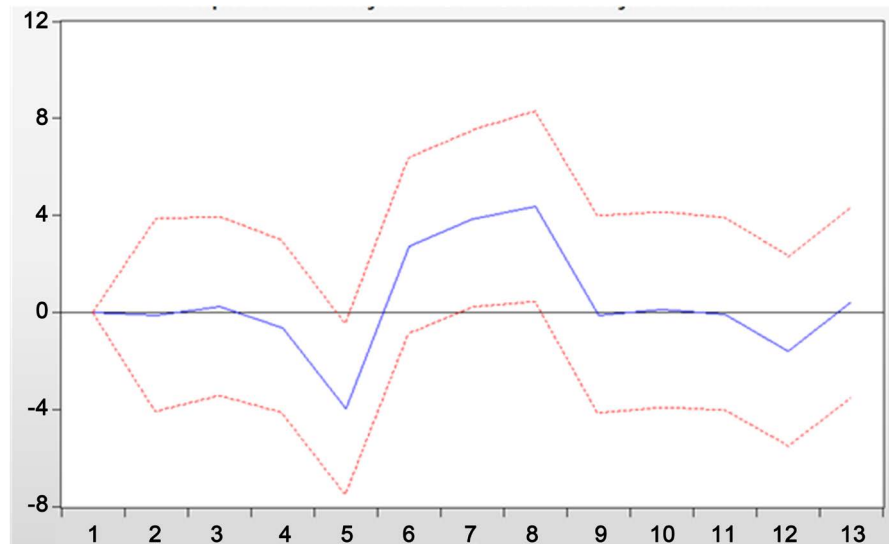
Figure 7. IRF—Industrial production on copper price.
