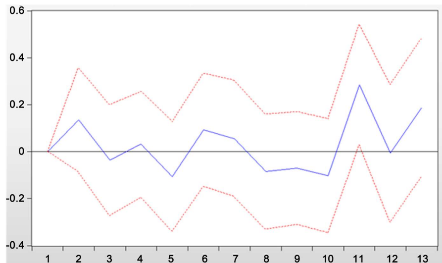
Figure 3. IRF—Brent price on copper price.
