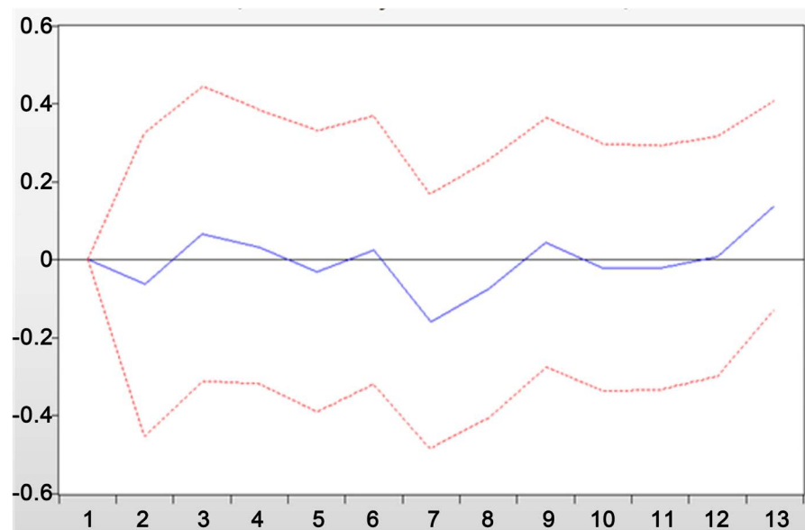
Figure 5. IRF—Copper stocks on copper price.
