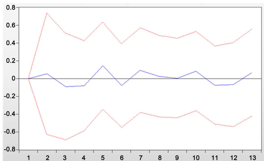
Figure 2. IRF—Copper production on copper price.
