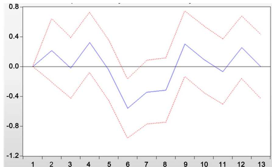
Figure 4. IRF—Aluminum price on copper price.
