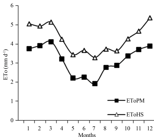
Figure 2. Comparison of mean monthly EToPM and EToHS and methods in São João, Pernambuco, Brazil, during the year of 2011.
