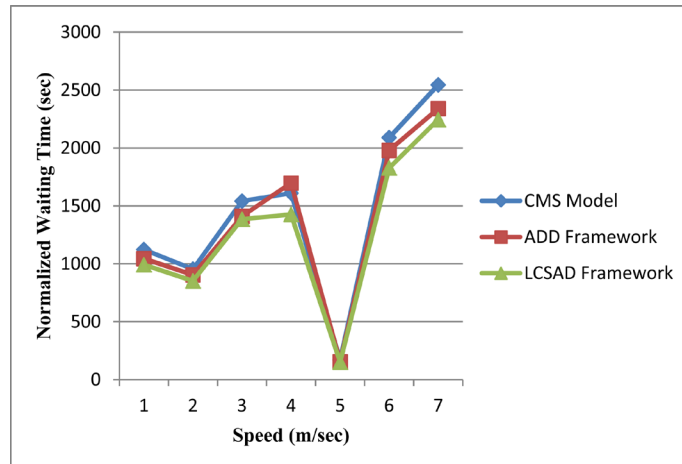
Figure 6. Measure of normalized waiting time.
