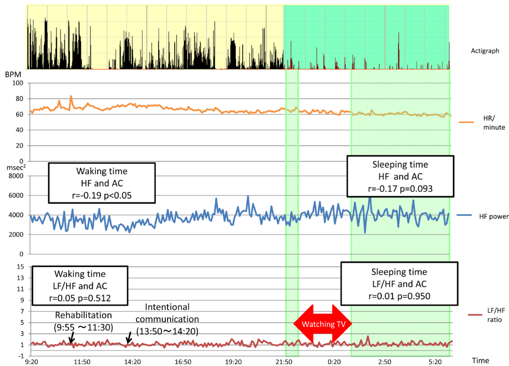
Figure 5. Typical example of no correlation between LF/HF and AC in PD subject No. 3 during sleeping time.
