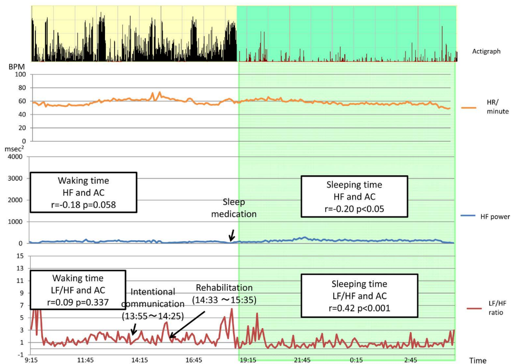
Figure 4. Typical example of significant positive correlation between LF/HF and AC in PD subject No. 5 during sleeping time.
