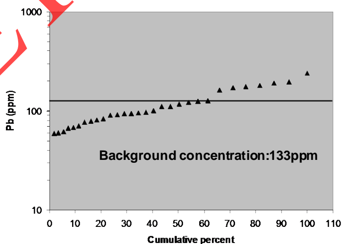
Figure 2. Cumulative-frequency curve used to determine the background concentration of lead.
