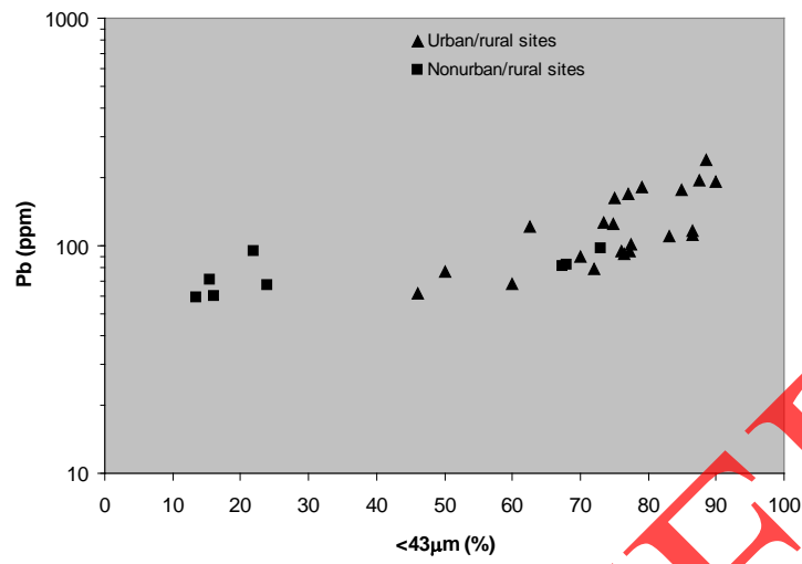
Figure 5. Comparison between trace-element concentrations and percent <43 µm particles for lead.
