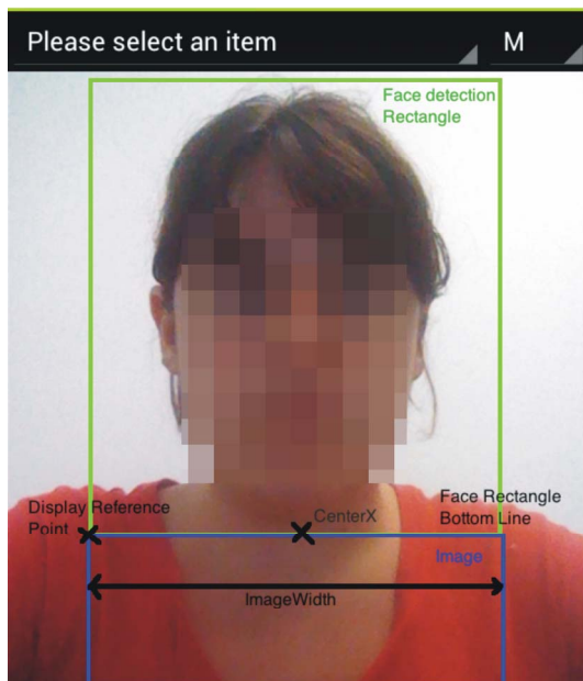
Figure 13. Calculations for the position.
