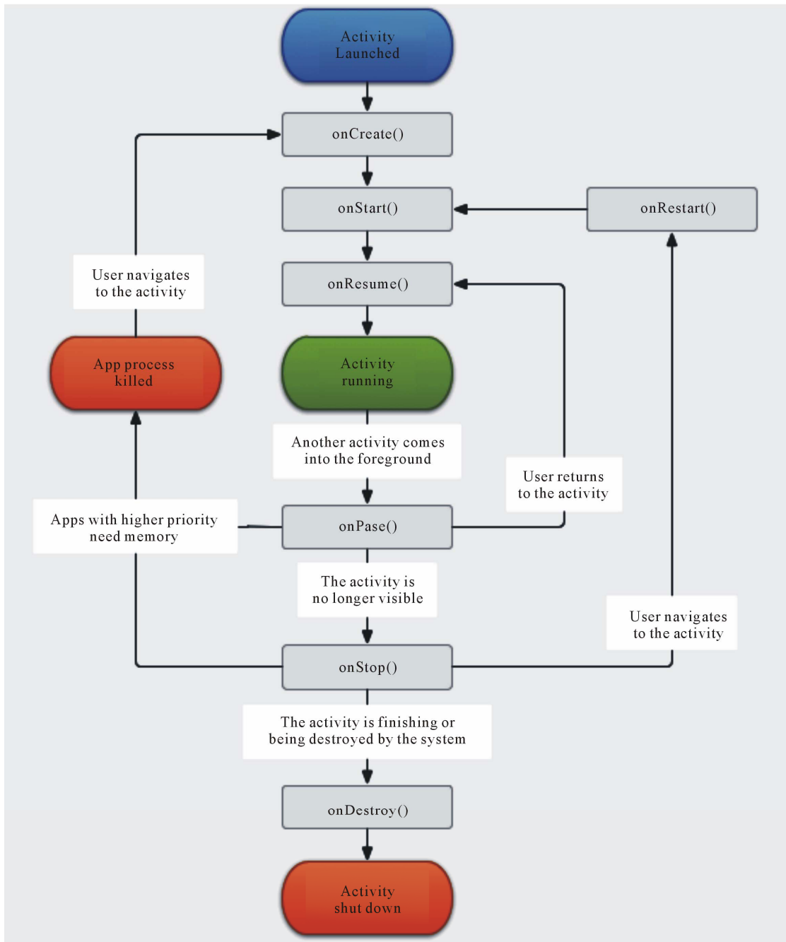
Figure 14. Android activity lifecycle.
