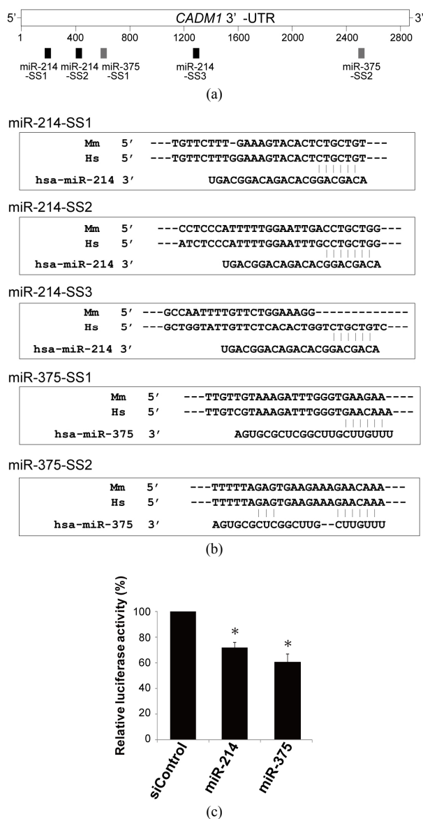
Figure 1. Targeting CADM1 by miR-214 and miR-375. (a) Predicted binding sites for the seed sequences of miR-214 and miR-375 in the 3'-UTR of CADM1 ; (b) Sequence alignments of miR-214 and miR-375 with 3'-UTR of CADM1 as indicated in A. The species abbreviations are Hs: Homo sapiens ; Mm: Mus musculus ; (c) Suppression of the luciferase activity of luciferase-CADM1 3'-UTR reporter gene by miRNA mimics of miR-214 and miR-375. Data are the mean \pm SEM of four independent experiments in duplicate. * p < 0.01 .
