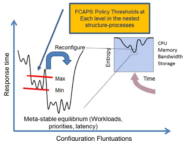
Figure 5. Meta-stable equilibriums.
